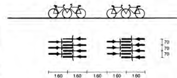
12 Front wheel overlapping with central access
