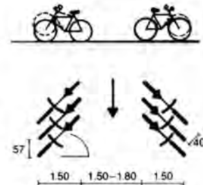
8 Staggered, herringbone formation
