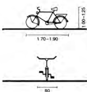
1 Basic bicycle dimensions
