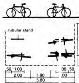
9 With tubular stands
