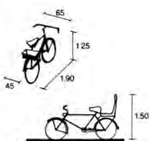
2 Bicycle with basket/child's seat
