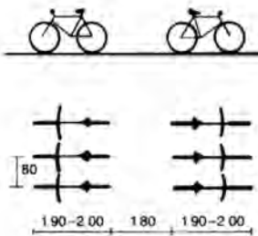
5 Basic layout parallel in straight lines
